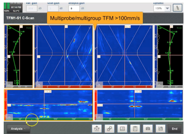
Figure 4: Multi-group and multi-mode TFM configurations.
